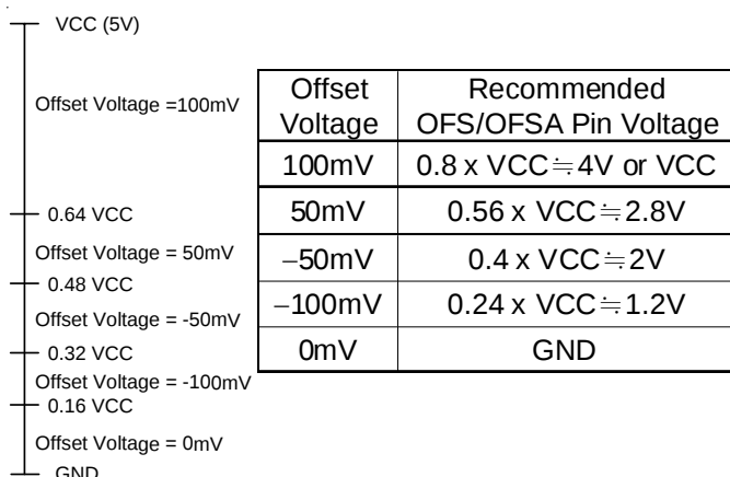
Figure 13. OFS and OFSA Pins Voltage Setting
