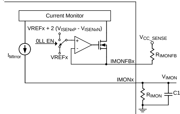
Figure 15. Current Monitor Setting Principle
