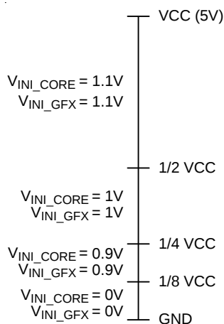
Figure 6. SETINI and SETINIA Pin Voltage Setting
