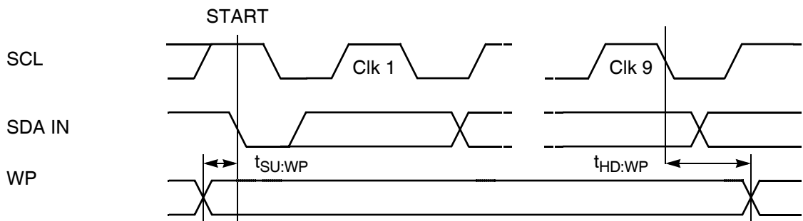
Figure 23. WP Pin Timing
