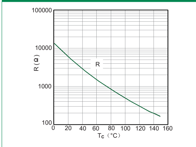
Figure 14: NTC Characteristics
