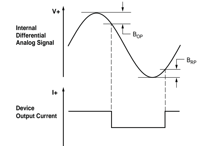
Figure 6: Peak Detecting Switchpoint Detail
