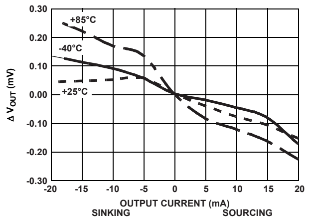
FIGURE 11. LOAD REGULATION
