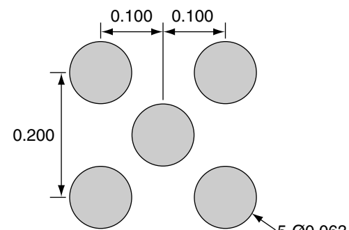
RECOMMENDED FOOTPRINT
