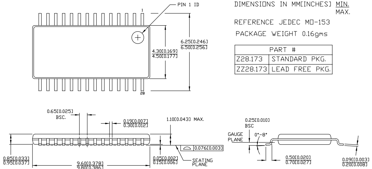
Figure 8. 28-pin TSSOP (4.40 mm Body) Package Outline, 51-85120
