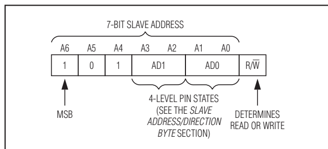
Figure 1. Slave Address
