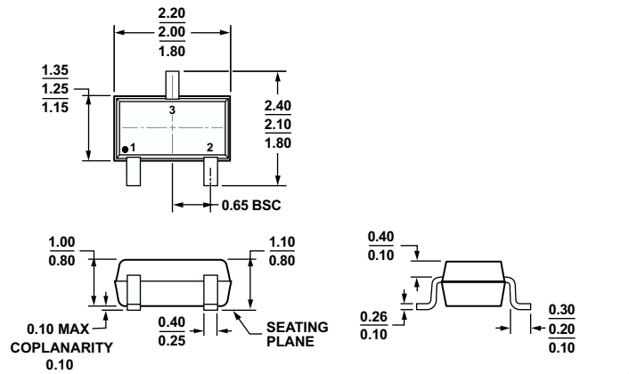
Figure 24. 3-Lead Thin Shrink Small Outline Transistor Package [SC70] (KS-3)
