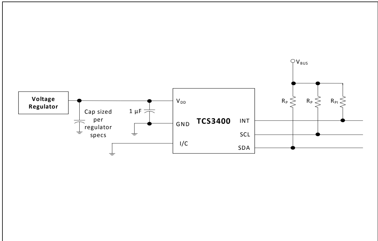
Figure 34: Typical Application Hardware Circuit
