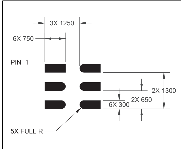
Figure 35: Suggested PCB Layout
