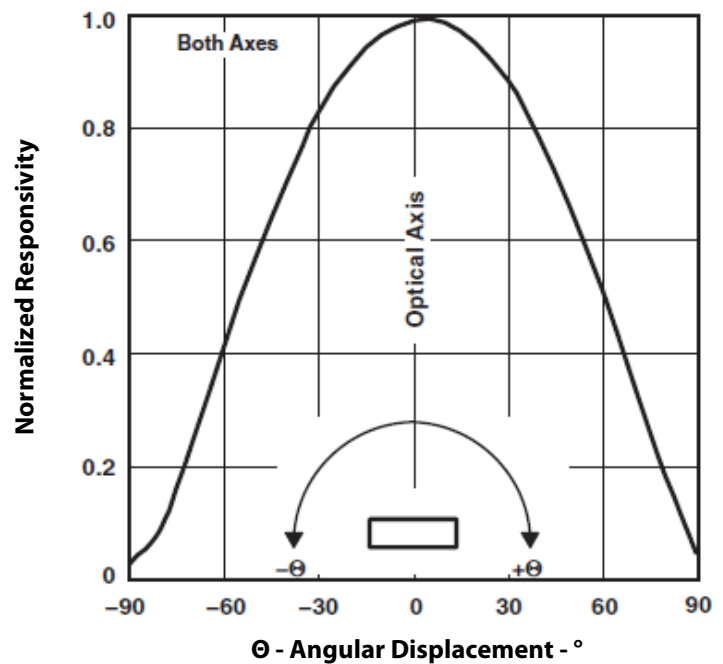
Figure 16: Normalized Responsivity vs. Angular Displacement
