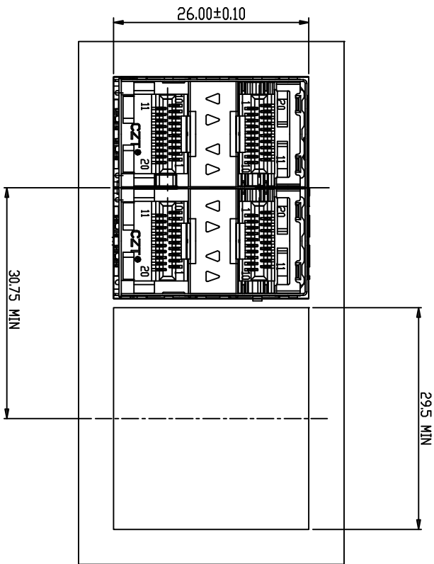
BEZEL CUT-OUT CENTER SPACING DETAIL BEZEL THICKNESS:0.8-2.6
