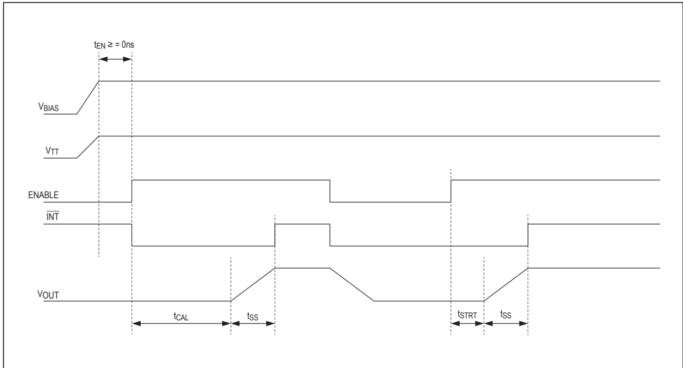
Figure 7. Startup Sequence
