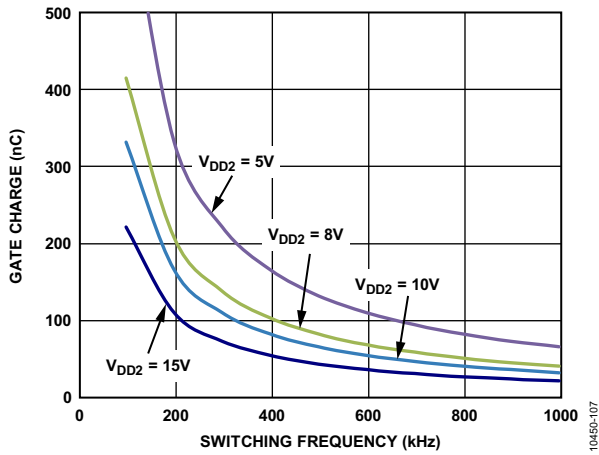
Figure 7. Typical ADuM3223 Maximum Load vs. Frequency ( R_G = 1 \Omega )
