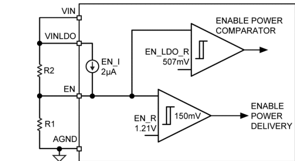
Figure 5. Programmable External UVLO Function
