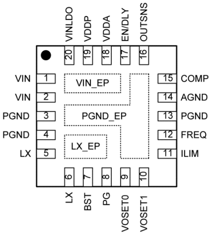
20–Pin 3mm × 3mm QFN (FL) (Top View)
