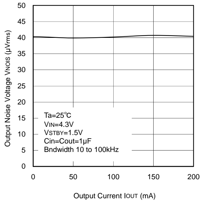
Figure 83. Output Noise Voltage vs. Output Current
