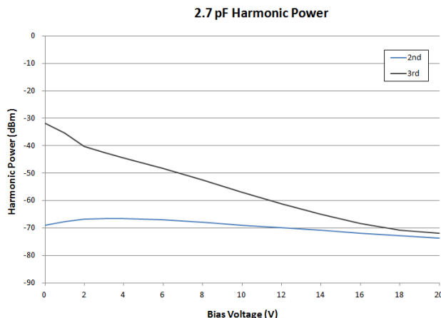
Figure 2. Harmonic Power
