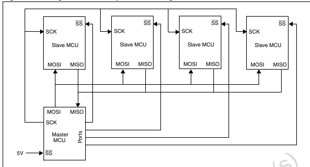
Figure 52. Single master/multiple slave configuration
