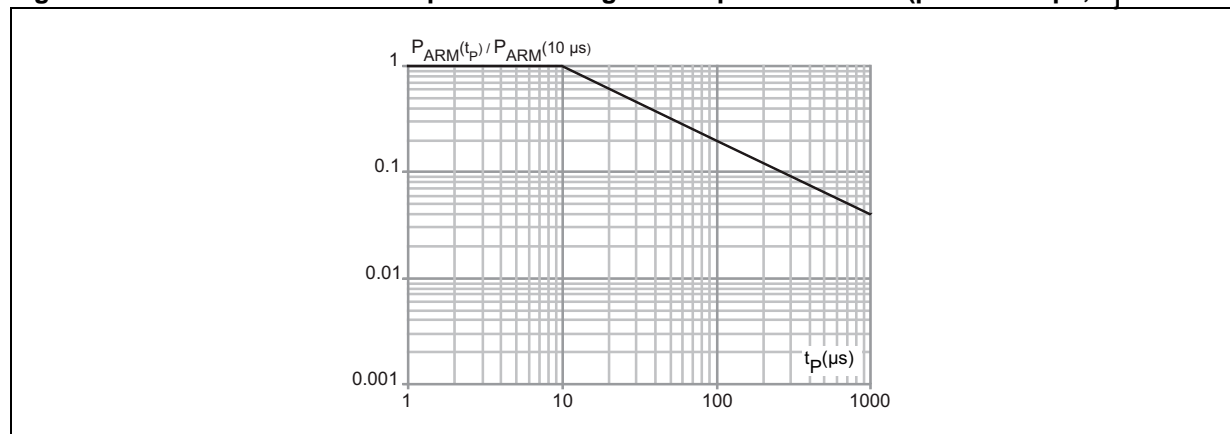
Figure 11. Normalized avalanche power derating versus pulse duration (pulse > 10 µs, T_J < 150 °C)
