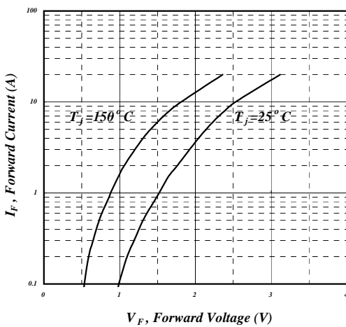
Fig 11. Forward Characteristic of Diode
