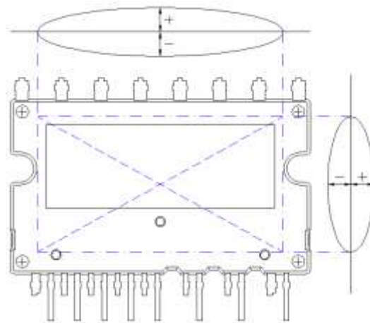
Figure 7: Flatness measurement position
