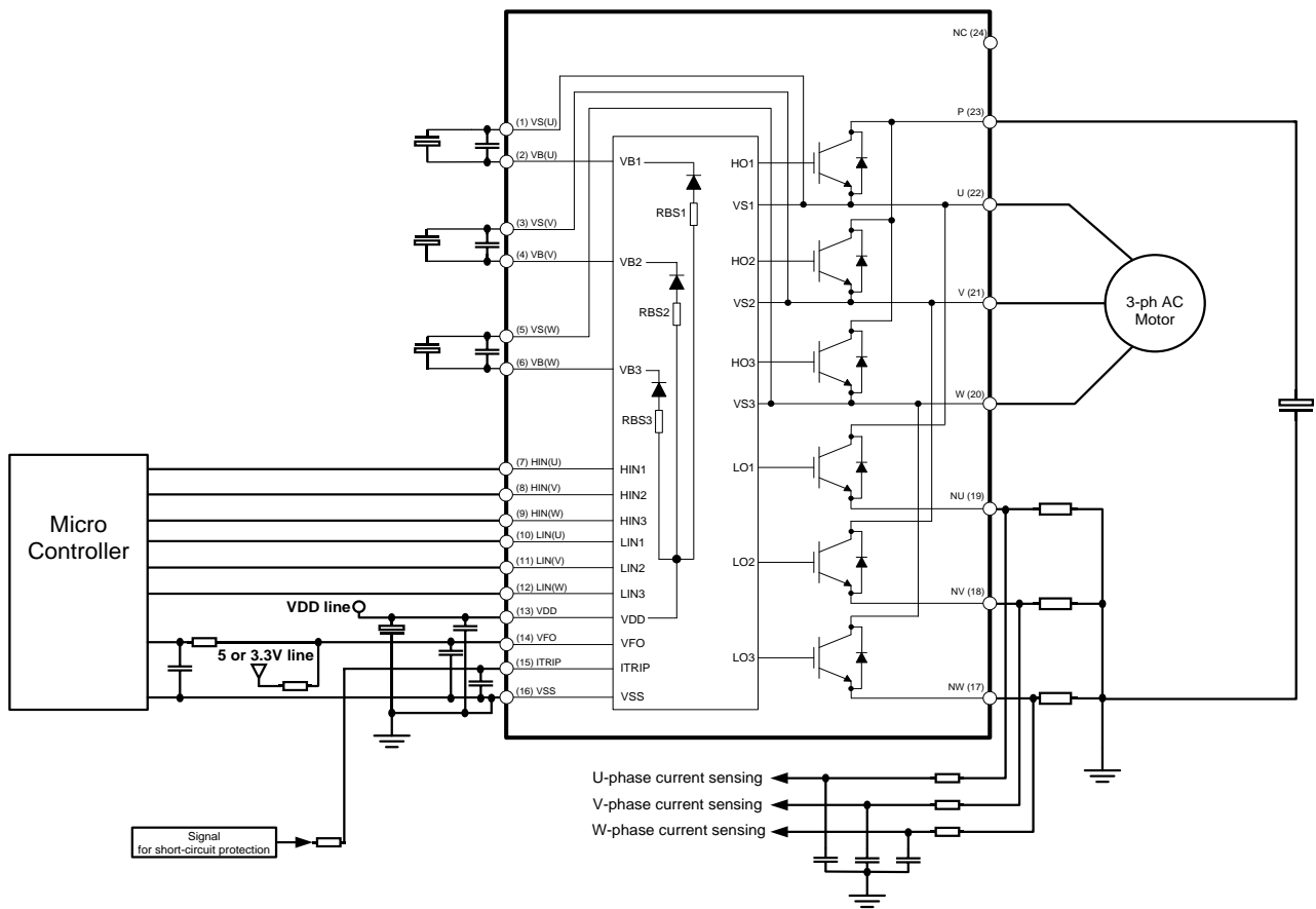
Figure 8: Application circuit
