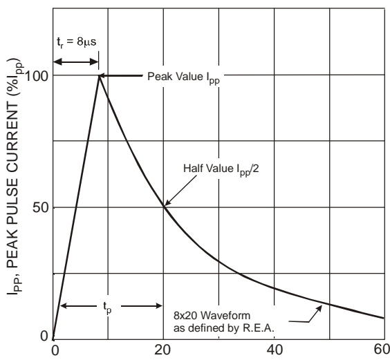
Figure 1 Pulse Waveform
