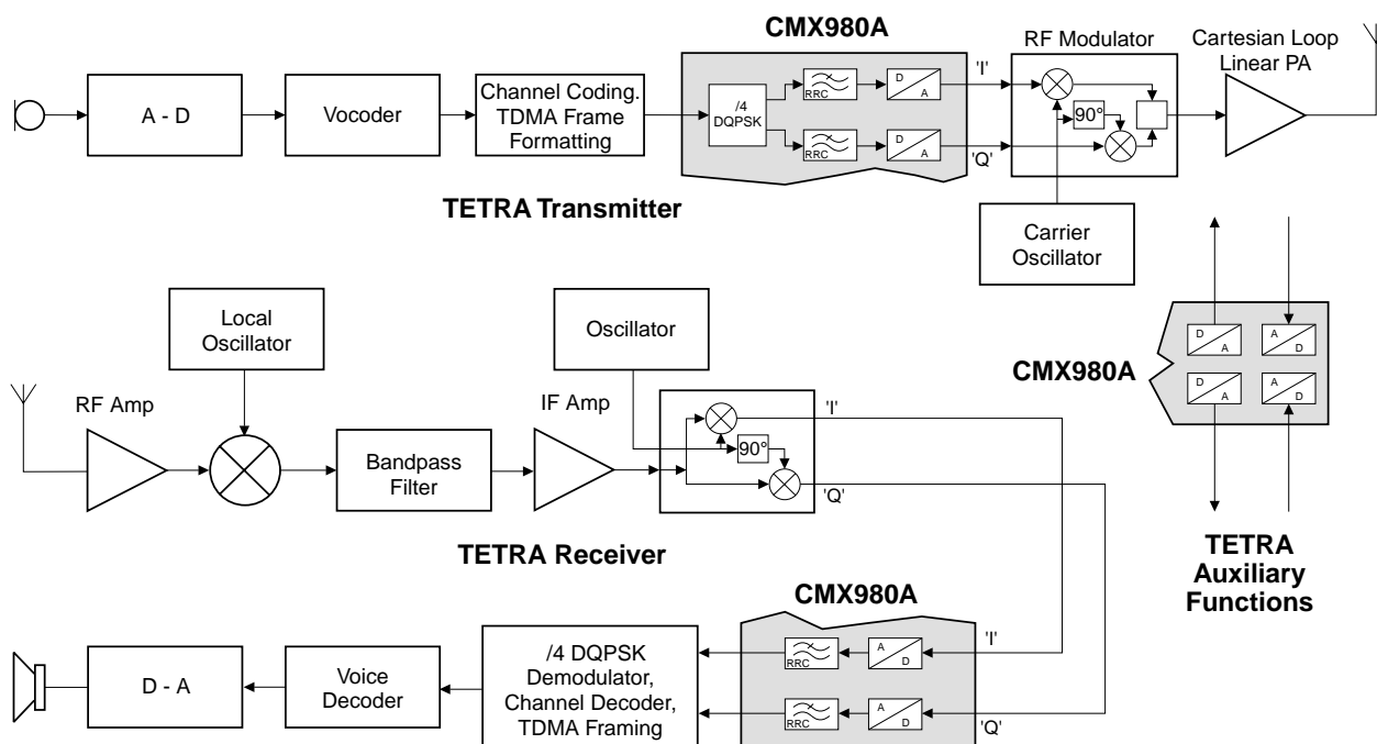
Example: CMX980A in a TETRA System Application
