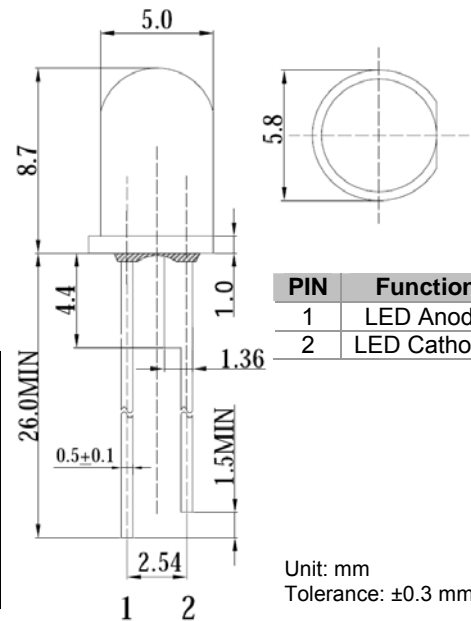
Outline Dimension:
