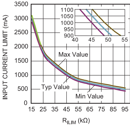
Input Current Limit vs. R_{LIM}
