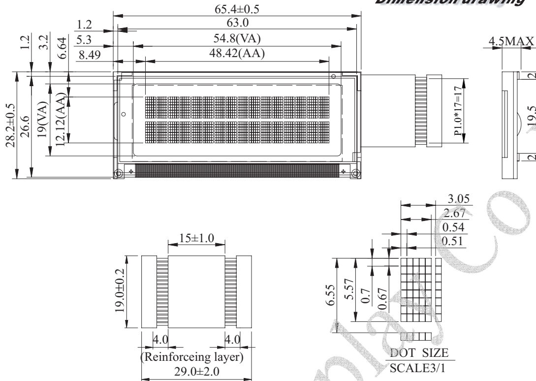
Dimension drawing
