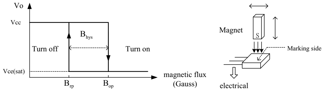
Fig.1 Hall-effect switch
