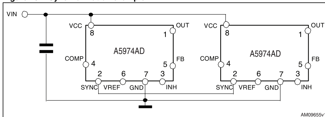
Figure 29. Synchronization example
