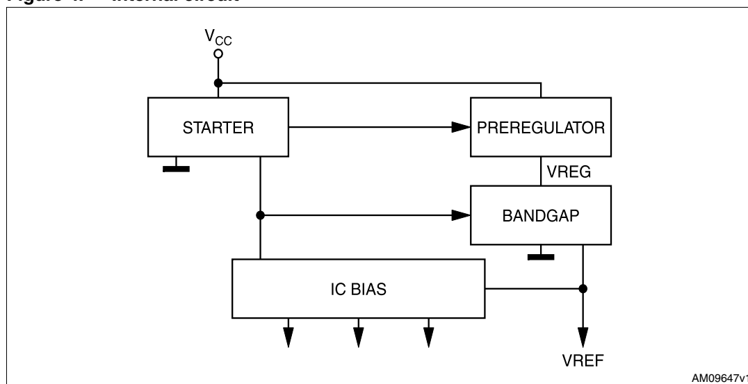
Figure 4. Internal circuit
