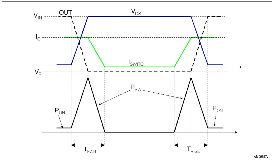
Figure 14. Switching losses
