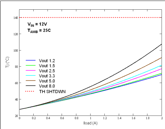
Figure 36. Junction temperature vs. output current ( V_{IN} = 12\text{ V} )
