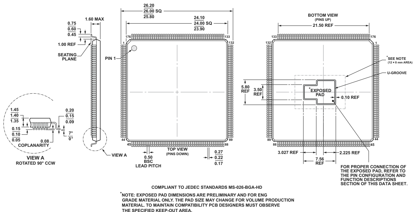
Figure 70. 176-Lead Low Profile Quad Flat Package, Exposed Pad [LQFP_EP] 1 (SW-176-3)
