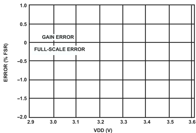
Figure 30. Gain Error and Full-Scale Error vs. Supply
