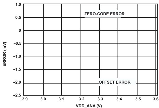
Figure 27. Zero-Code Error and Offset Error vs. Supply
