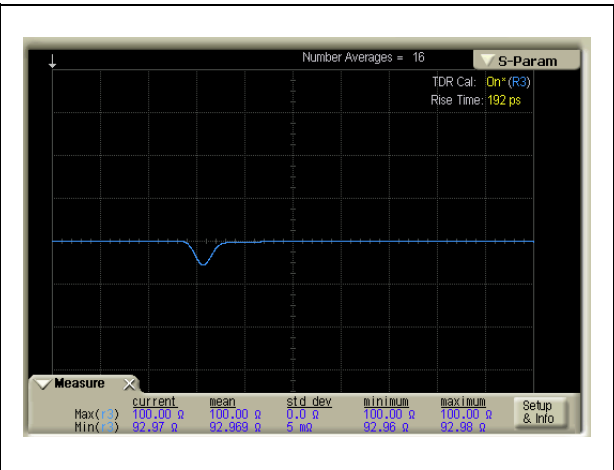
Figure 15. TDR measurement
