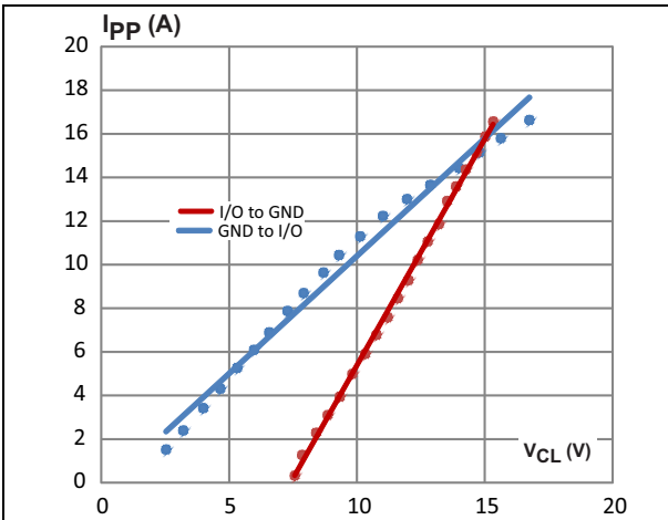
Figure 14. TLP measurement (pulse duration 100 ns)
