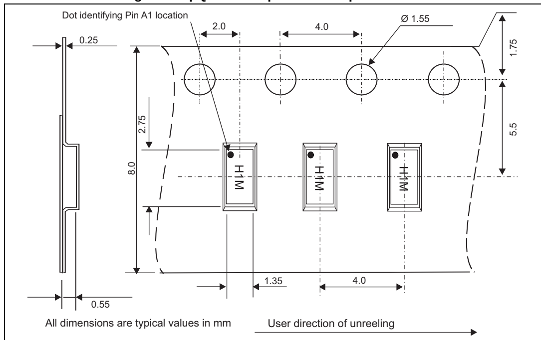
Figure 19. \mu QFN-10L tape and reel specification
