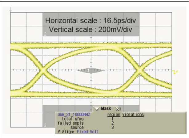
Figure 11. Eye diagram - USB 3.1 mask at 10.0 Gbps per channel (with HSP051-4M10)
