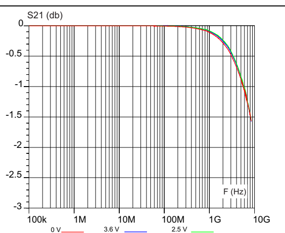
Figure 3. S21 attenuation measurement
