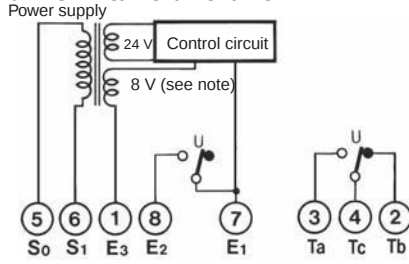
61F-GP-N8/-N8L/-N8D/-N8HY Power supply
