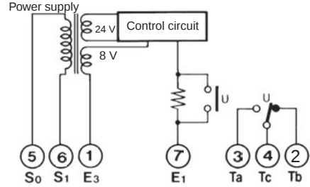
61F-GP-N8R Power supply
