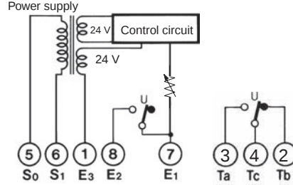
61F-GP-N8-V50 Power supply
