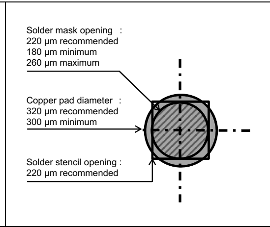
Figure 14. Recommended land pattern
