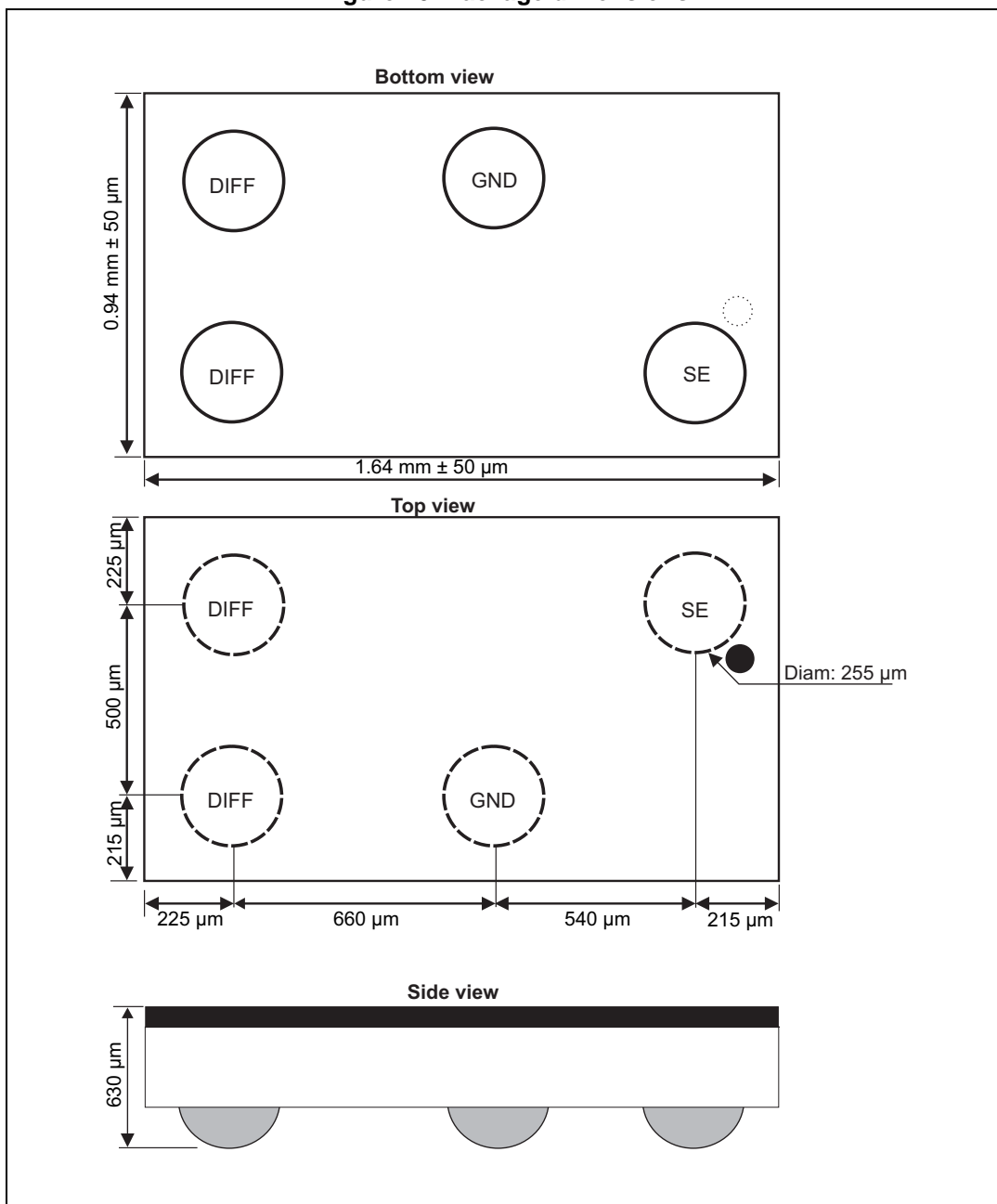
Figure 10. Package dimensions
