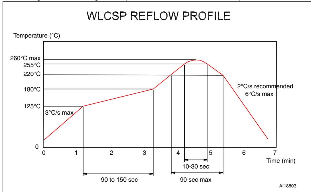
Figure 7. Soldering reflow profile used for all ST WLCSP qualifications
