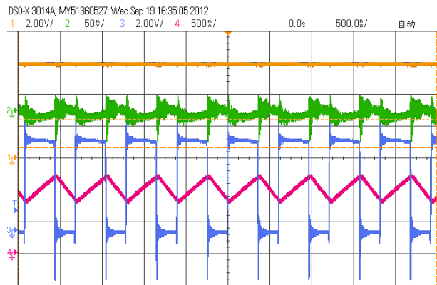
Ch1: Vin, Ch2: Vout, Ch3 SW, Ch4: I_inductor
