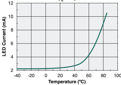
Typical I_F for Switch Operation vs. Temperature ( I_L=1\text{A} )
