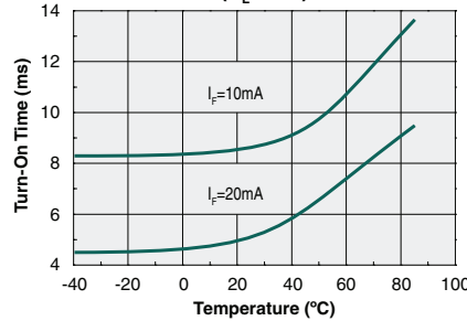
Typical Turn-On Time vs. Temperature ( V_L=10\text{V} )
