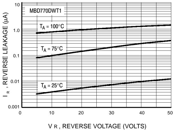
Figure 12. Reverse Leakage
