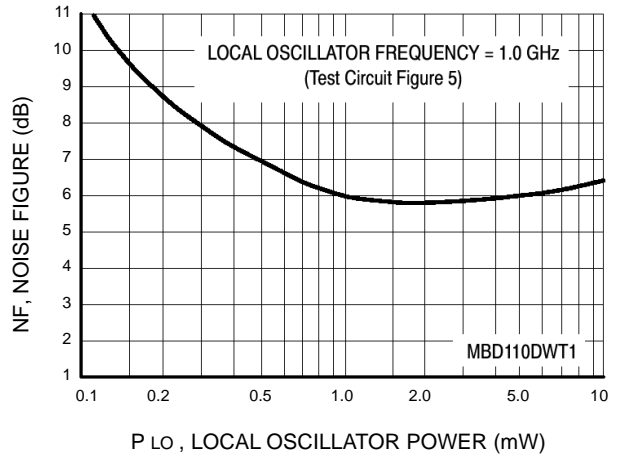
Figure 4. Noise Figure
