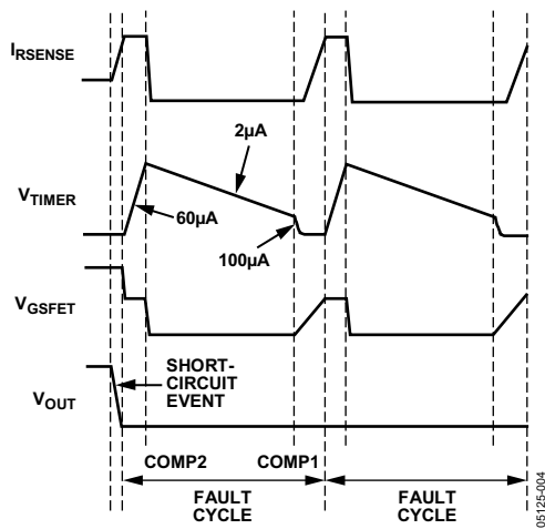
Figure 38. ADM1171-1 Automatic Retry During Overcurrent Fault
