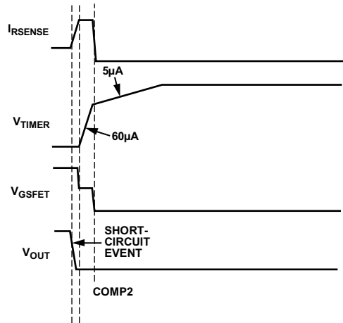
Figure 39. ADM1171-2 Latch Off After Overcurrent Fault
