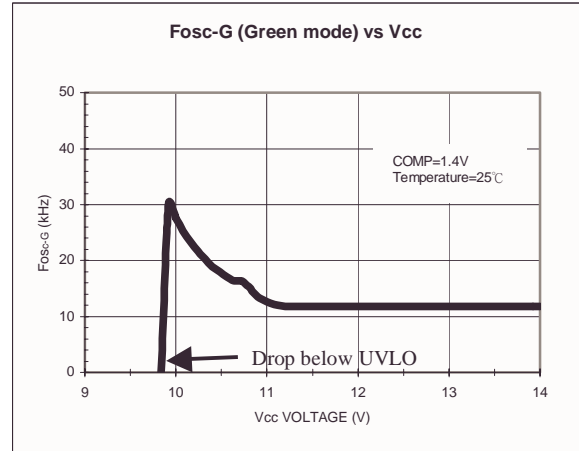
Fig.2 Green-mode Frequency vs. Supply Voltage V_{cc}
