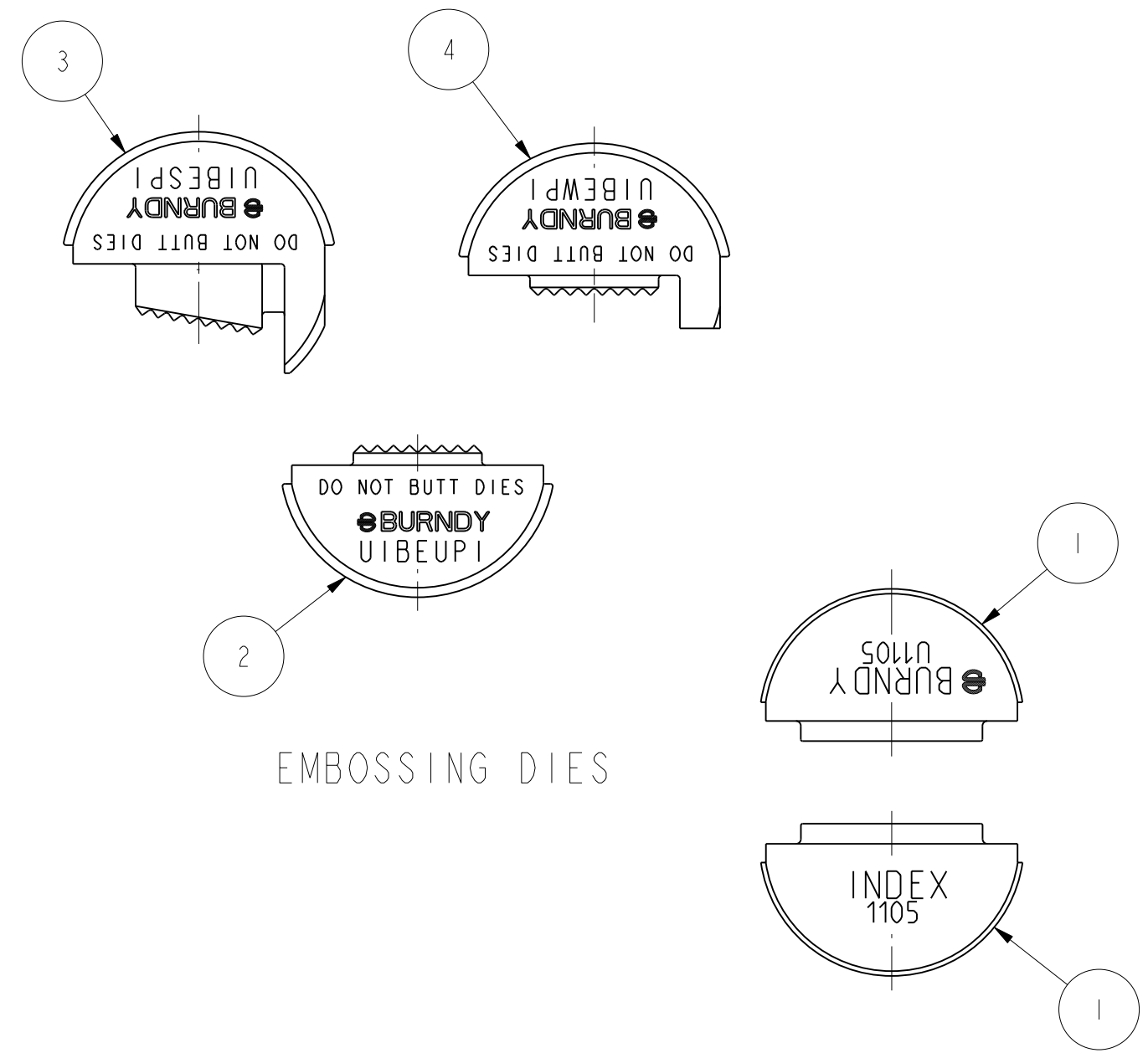
CRIMPING DIES
