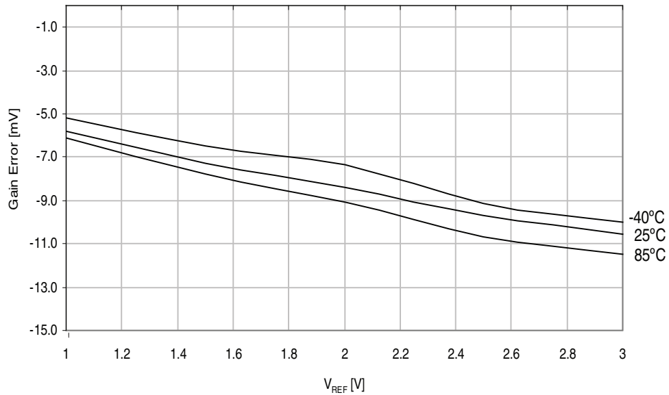
Figure 37-32. ADC Gain Error vs. V_{REF} . Differential signed mode, external reference.
