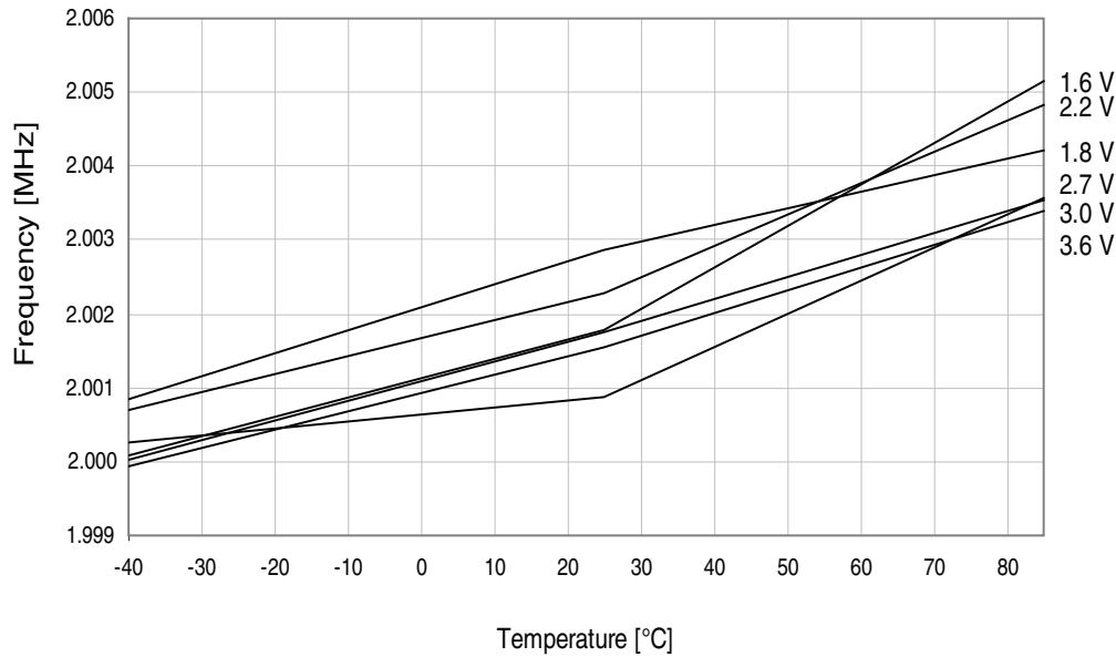
Figure 37-62. 2MHz internal oscillator frequency vs. temperature. DPLL enabled.
