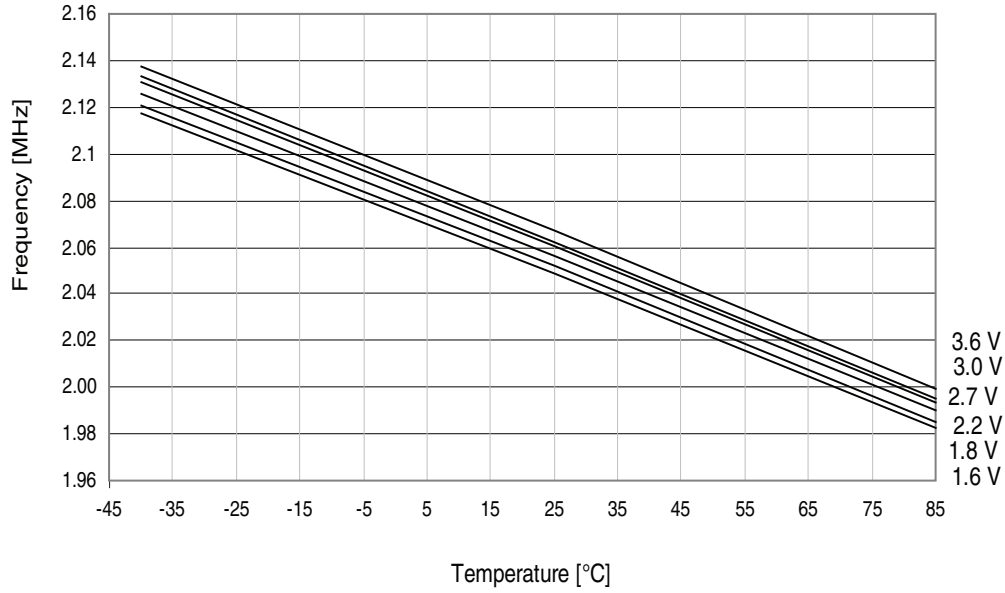
Figure 37-61. 2MHz internal oscillator frequency vs. temperature. DPLL disabled.
