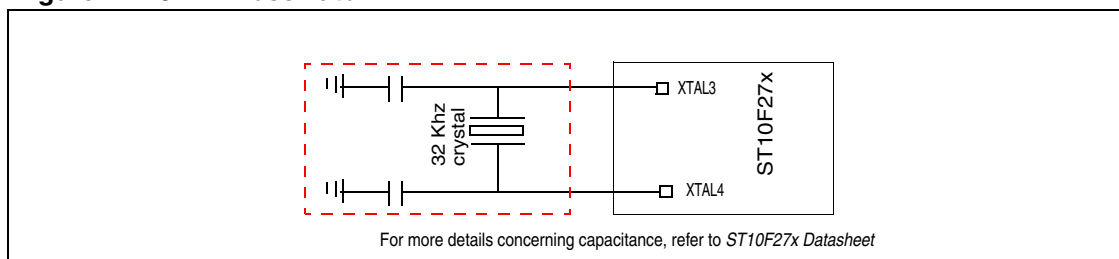
Figure 4. 32 kHz oscillator
