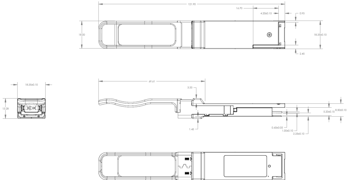
Figure 2 – FTL414QB2C mechanical drawing
