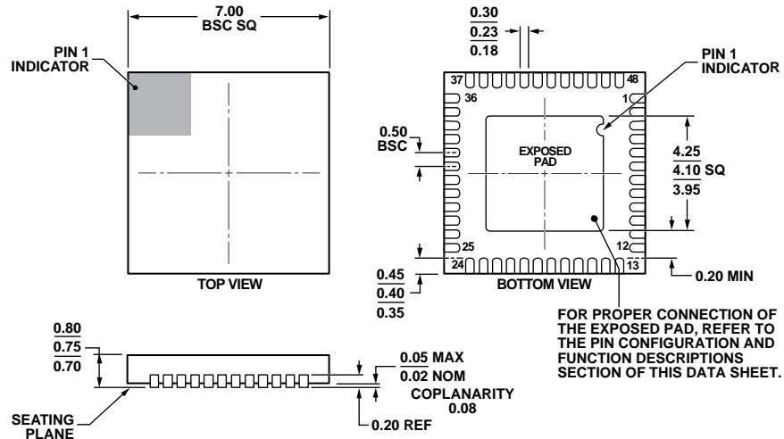
Figure 30. 48-Lead Lead Frame Chip Scale Package [LFCSP_WQ] 7 mm × 7 mm Body, Very Thin Quad (CP-48-5) Dimensions shown in millimeters
