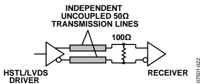
Figure 27. LVDS or HSTL Output Termination
