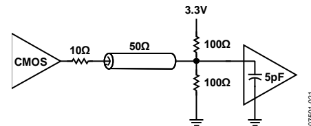
Figure 25. CMOS Output with Far End Termination
