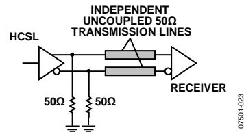
Figure 28. HCSL Output Termination
