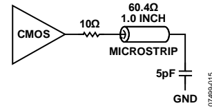
Figure 24. Series Termination of CMOS Output
