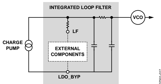
Figure 22. PLL Loop Filter Detail
