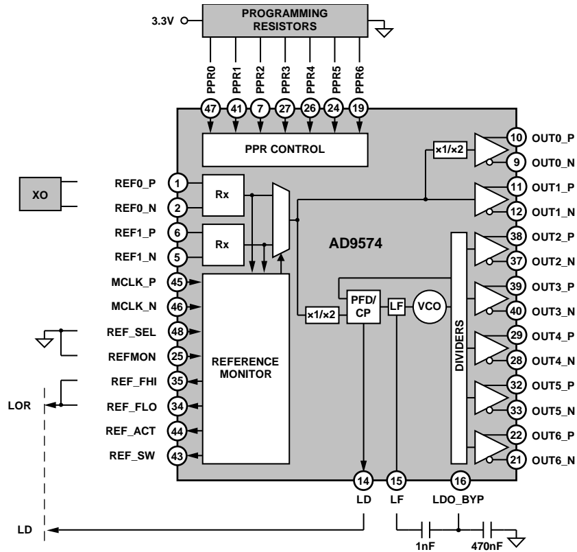
Figure 26. Single-Oscillator Reference Input Application Diagram
