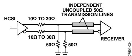
Figure 29. Alternate HCSL Output Termination
