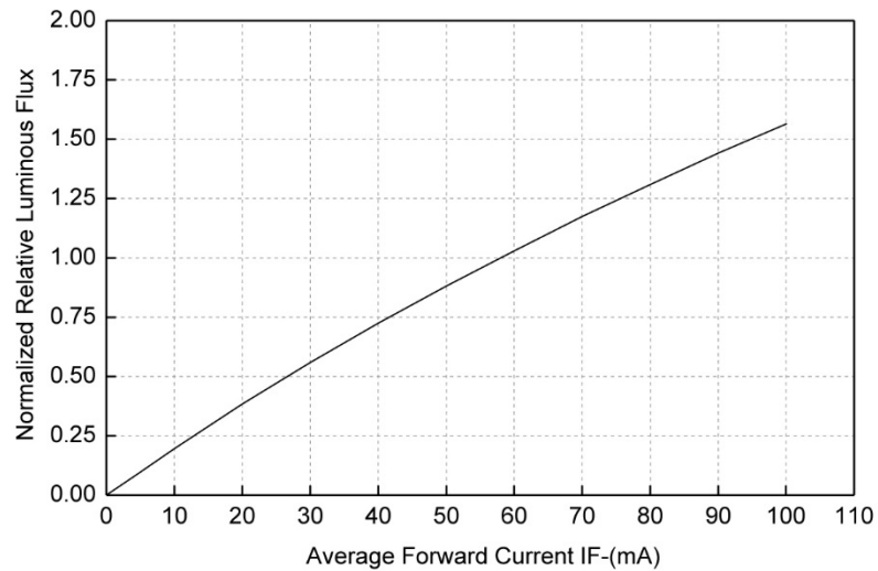
Figure2. Relative Luminous Flux VS. Forward Current
