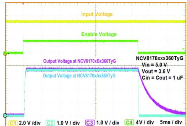
Figure 40. Load Transient Response at Load Step from 0.1 mA to 10 mA, V_{out} = 3.6\text{ V}
