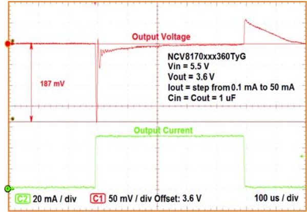
Figure 36. Load Transient Response at Load Step from 0.1 mA to 50 mA, V_{out} = 3.0\text{ V}
