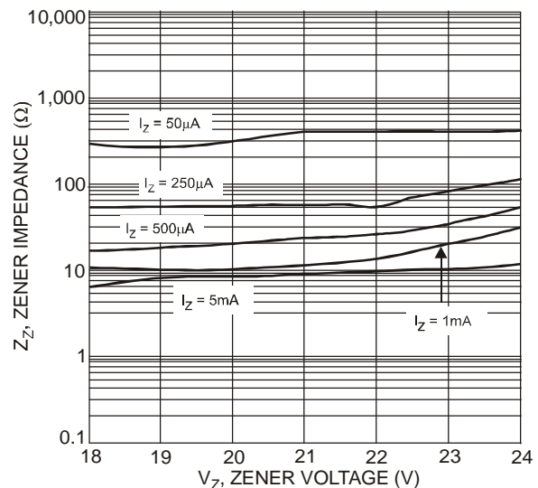
Fig. 13 Typical Zener Impedance Characteristics, DDZ18CS - DDZ24CS
