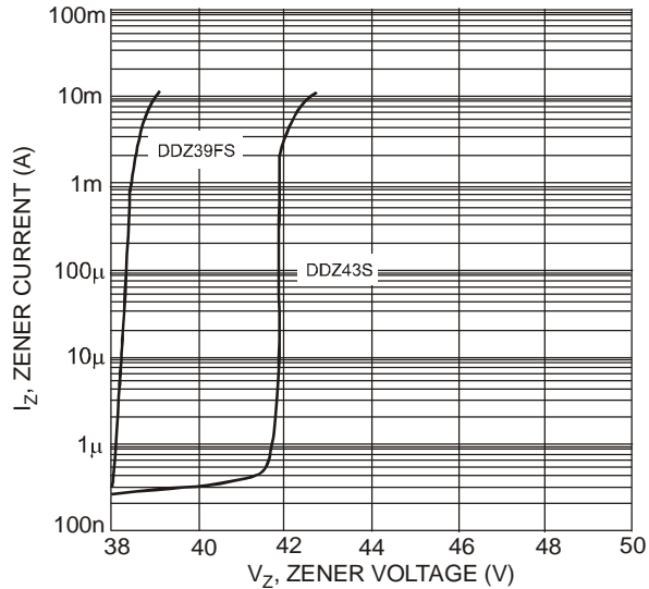
Fig. 9 Typical Zener Breakdown Characteristics, DDZ39FS - DDZ43S
