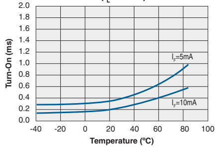
Typical Turn-On vs. Temperature (I L =80mA)
