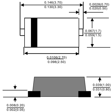
SOD-123
