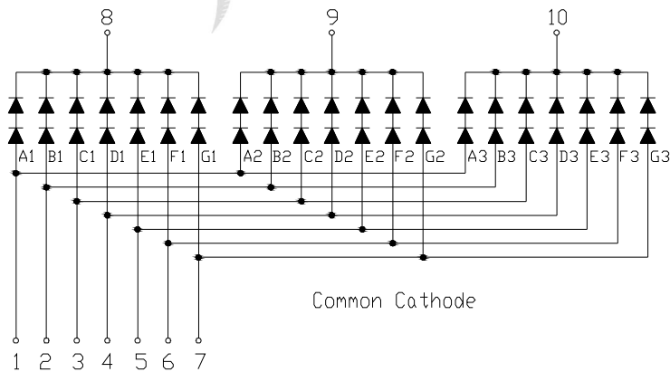
FYA-CR41AX
