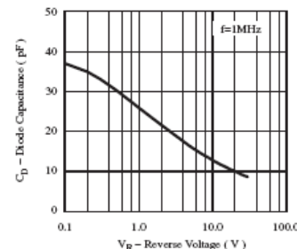
Typ. Diode Capacitance vs. Reverse Voltage
