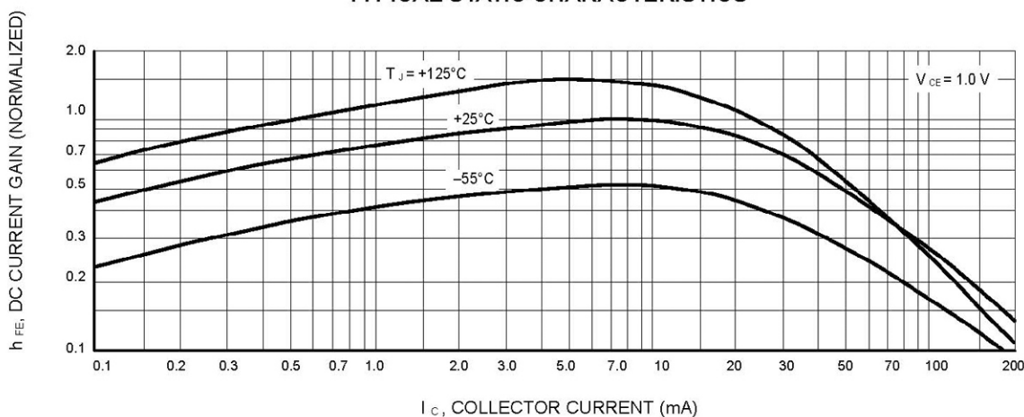
Figure 15. DC Current Gain
