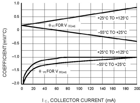
Figure 18. Temperature Coefficients
