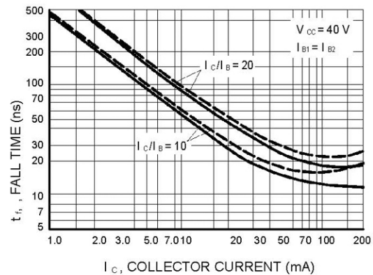
Figure 8. Fall Time
