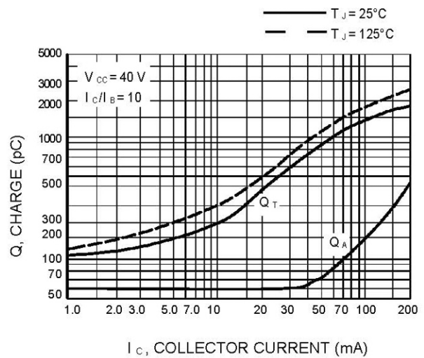
Figure 4. Charge Data
