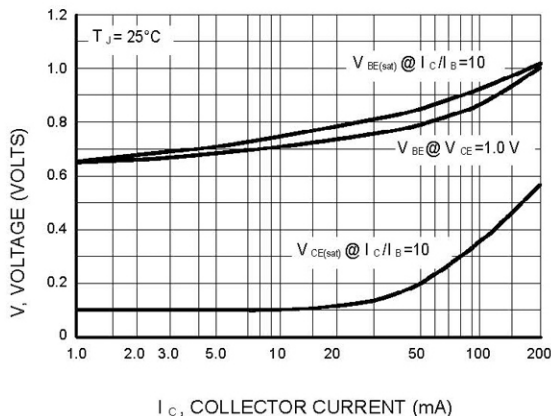
Figure 17. "ON" Voltages
