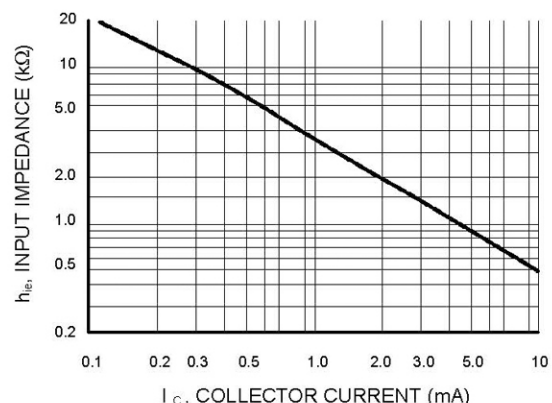
Figure 13. Input Impedance
