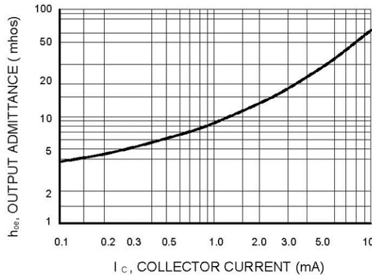
Figure 12. Output Admittance
